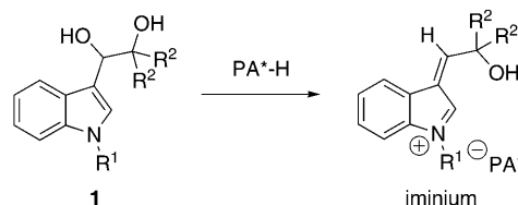
Scheme 1. Dehydration strategy for the chiral phosphoric acid catalyzed pinacol rearrangement.
