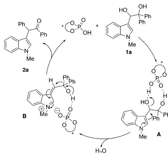
Scheme 2. Proposed mechanism for the chiral phosphoric acid catalyzed asymmetric pinacol rearrangement.
